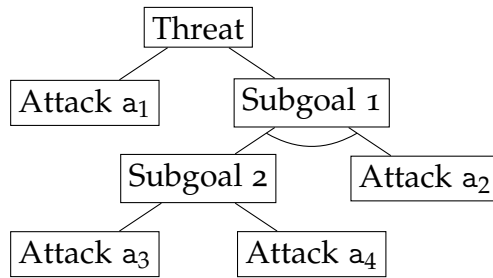
Figure 3.6.: Example attack tree.
