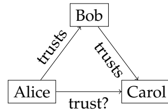
Figure 4.2.: Trust relations.
