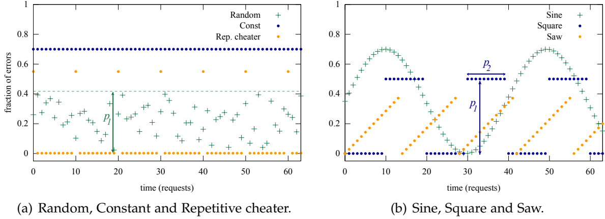
Figure 4.12.: Attack strategies that form the attack strategy search space.
