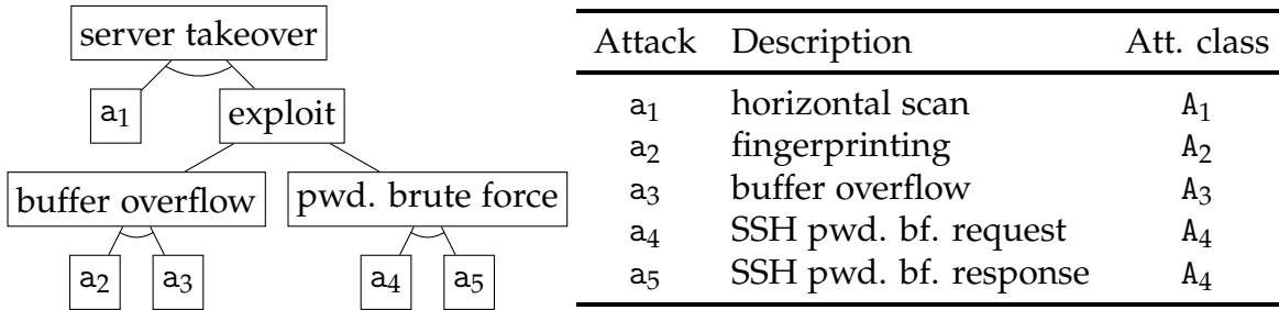
Figure C.1.: Example attack tree T_1 .
