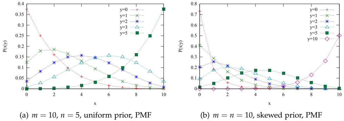
Figure 3.2.: Probability distributions for incorrect replies.
