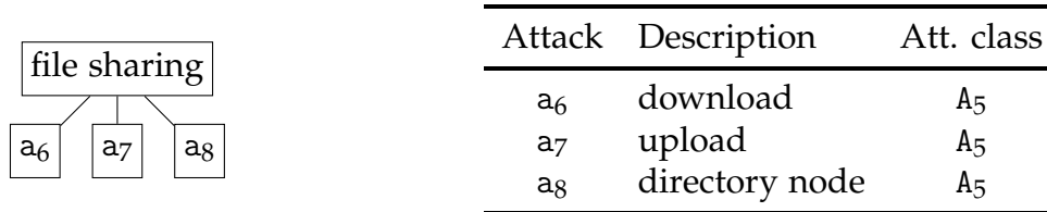
Figure C.2.: Example attack tree T_2 .
