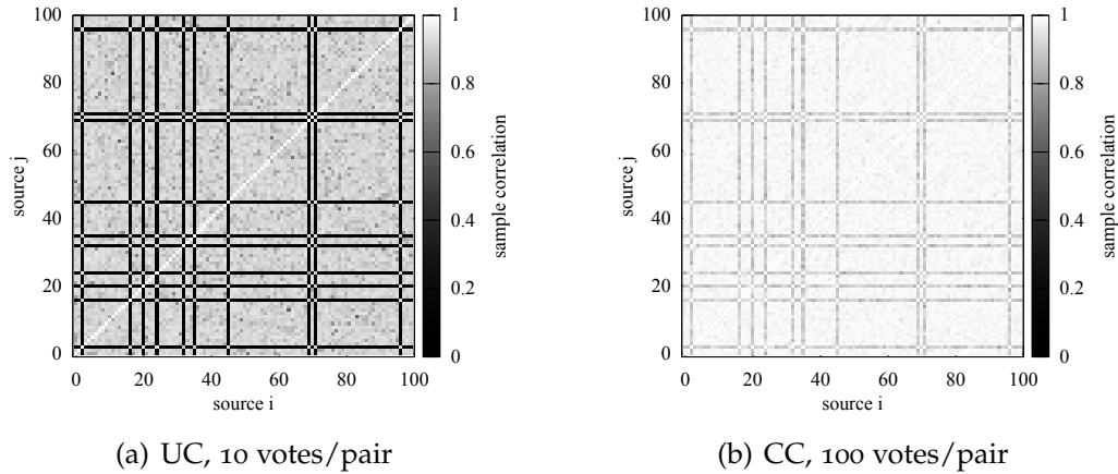
Figure 5.2.: Sample collusion matrices ( k = 3 , |\mathcal{S}| = 100 ).
