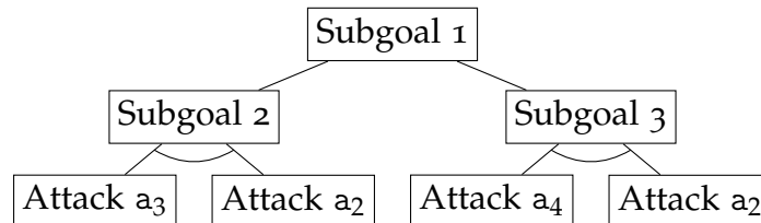
Figure 3.7.: Subtree.
