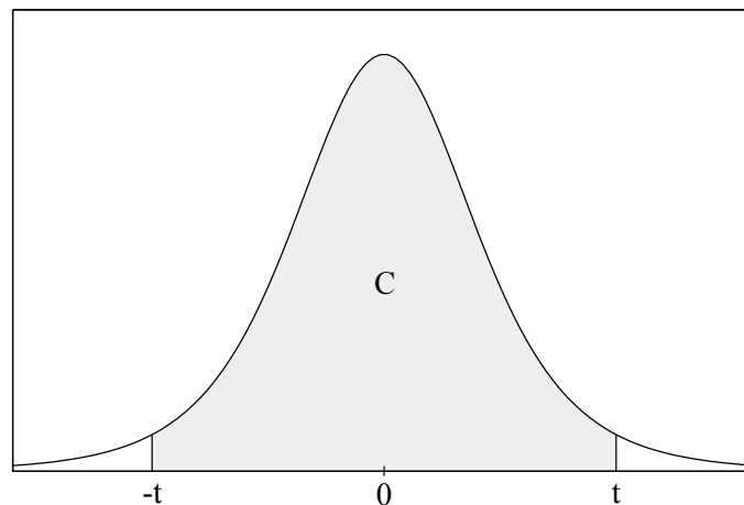
Figure B.1.: Critical values for a t-distribution.
