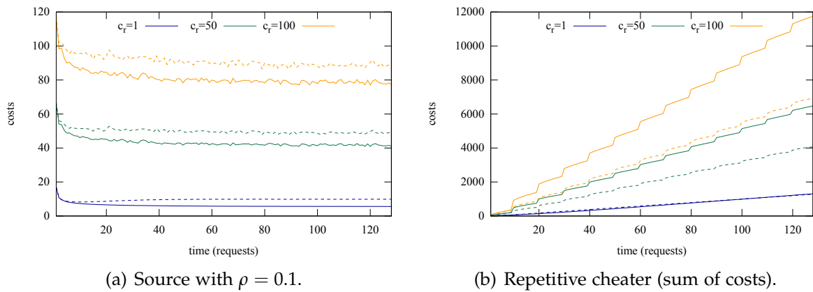
Figure 4.9.: Costs for flexible n for \epsilon = \frac{1}{7} (dashed), and \epsilon = \frac{2}{7} (solid) ( m = 10 , c_c = 1 ).
